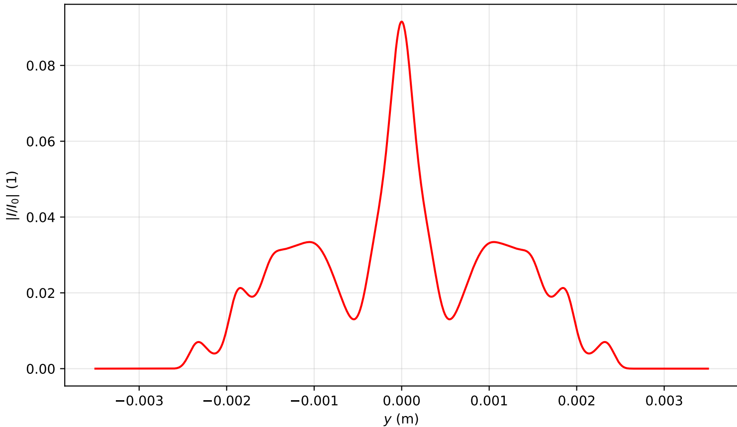
Intensity profile I(x=0, y, z=3.582)/I_0 , P_{in}=8.5P_{cr} , artificial time
